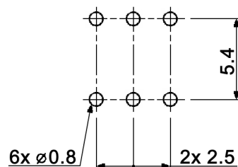
HOLE LAYOUT TOP VIEW \oplus 0.05
