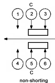
CIRCUIT DIAGRAM C: COMMON PIN BOTTOM VIEW
