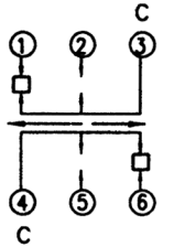
CIRCUIT DIAGRAM C:COMMON PIN BOTTOM VIEW
