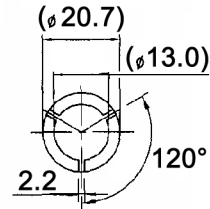
"A" DETAIL
