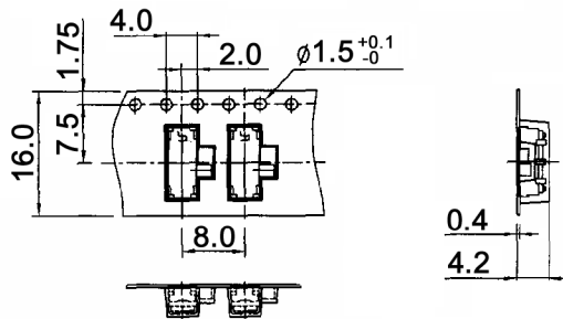
CARRIER TAPE
