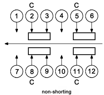
CIRCUIT DIAGRAM C: COMMON PIN BOTTOM VIEW
