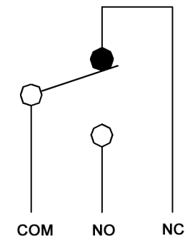
SCHMATIC
